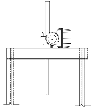
ELECTRIC ACTUATOR (Bench Mount)
