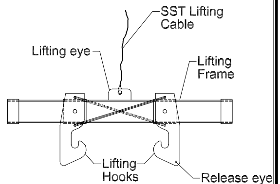
STOP LOG LIFTER
