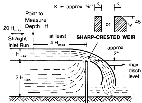
Figure B—Profile of Sharp-Crested Weir
