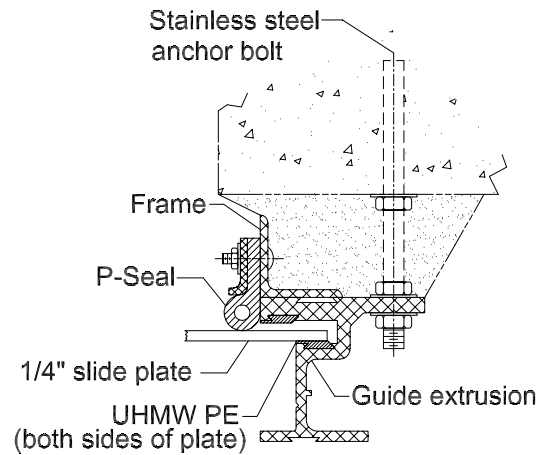
GUIDE FRAME Detail-A
