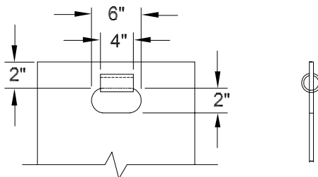
GATE WITH PIPE/HAND SLOT HANDLE
