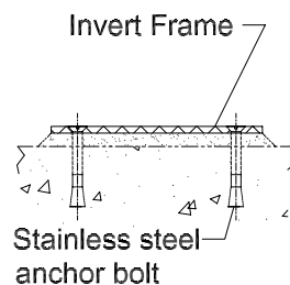
SURFACE MOUNT INVERT * Detail-C
