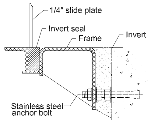
FLUSH BOTTOM INVERT * Detail-C
