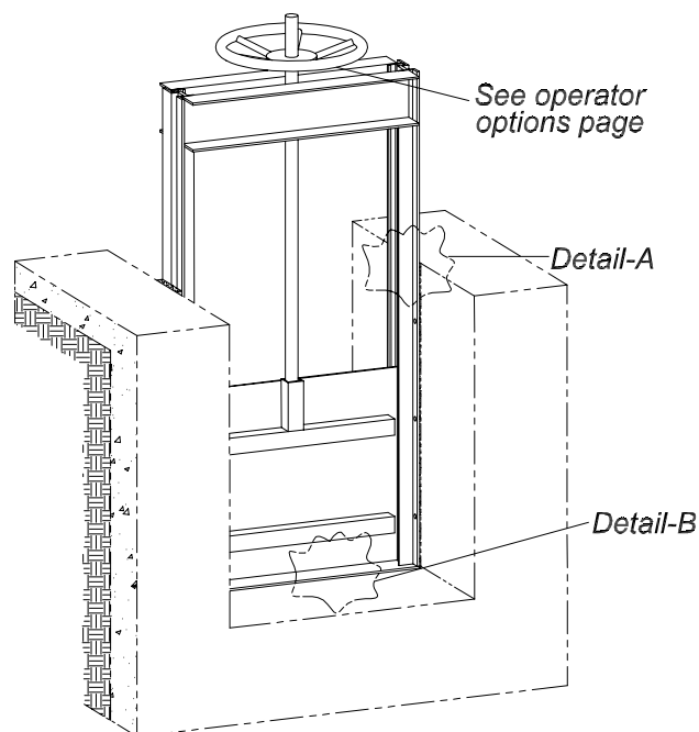
SELF-CONTAINED GATE WITH BENCH (YOKE)
