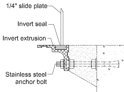
FLUSH BOTTOM INVERT * Detail-C
