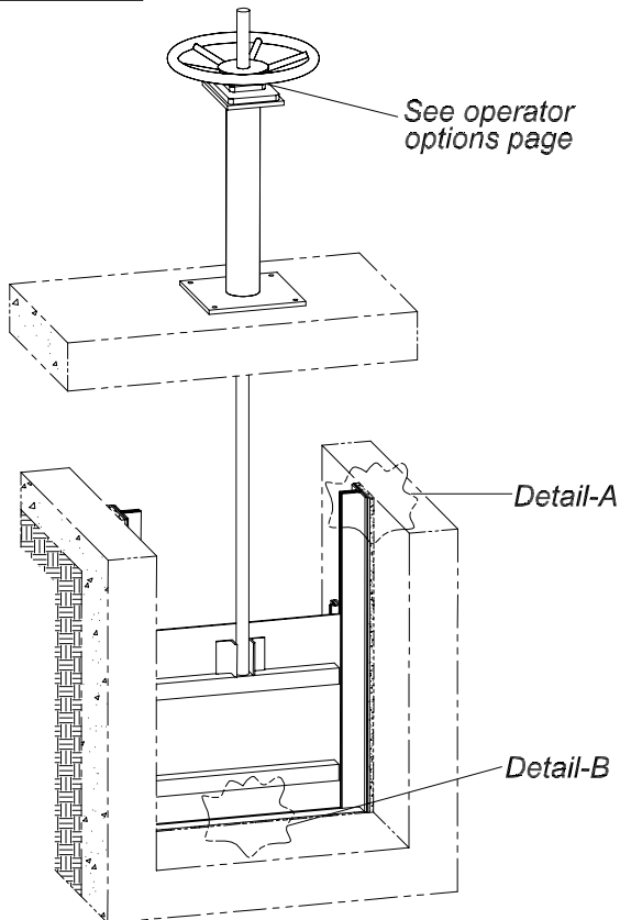
NON-SELF-CONTAINED GATE WITH FABRICATED PEDESTAL
