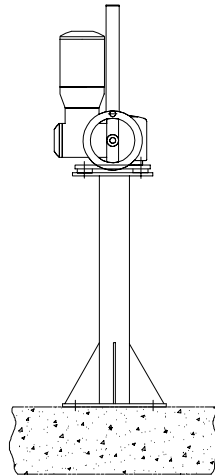
ELECTRIC ACTUATOR (Pedestal Mount)
