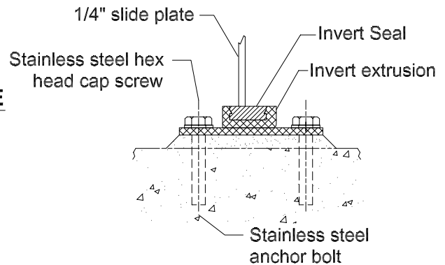
INVERT (OPTION 1) Detail-B
