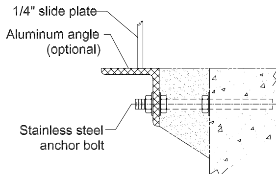
GATE STOP ANGLE (optional) Detail-C
