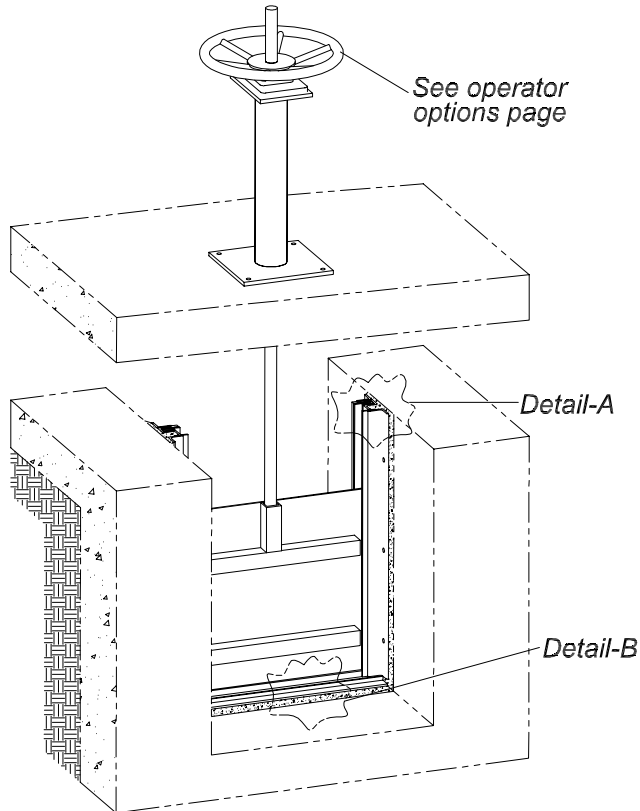
NON-SELF-CONTAINED GATE WITH FABRICATED PEDESTAL
