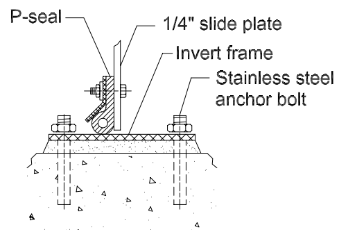
INVERT (OPTION 2) Detail-B
