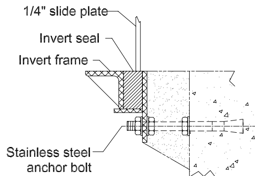
FLUSH BOTTOM INVERT Detail-C
