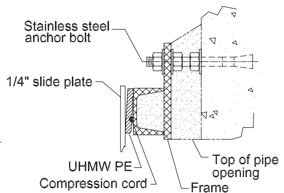
UPPER SEAL * Detail-B
