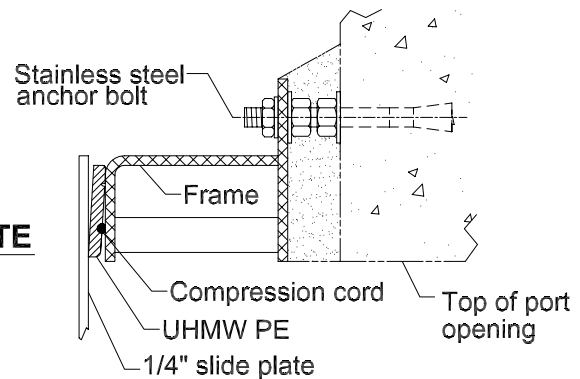
UPPER SEAL * Detail-B
