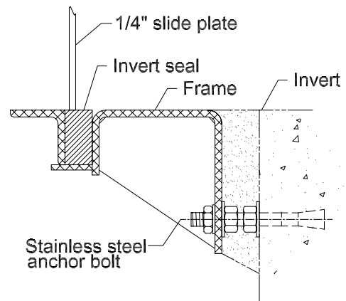
FLUSH BOTTOM INVERT * Detail-B
