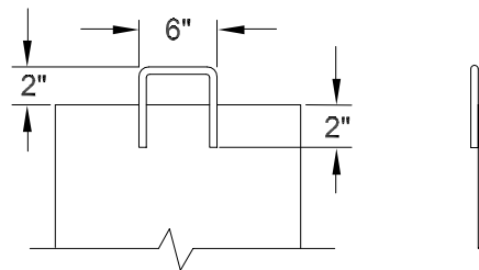
GATE WITH H-1 HANDLE
