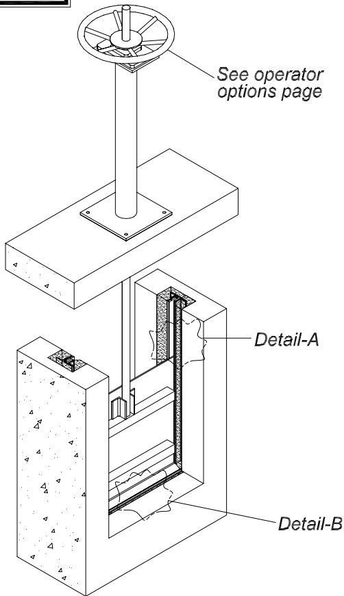
NON-SELF-CONTAINED GATE WITH FABRICATED PEDESTAL
