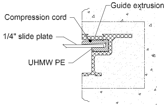
GUIDE FRAME Detail-A
