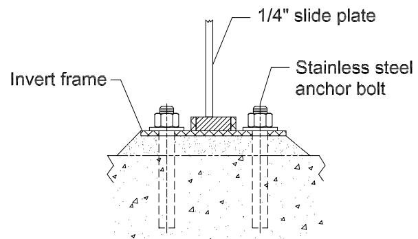
INVERT (OPTION 1) Detail-B
