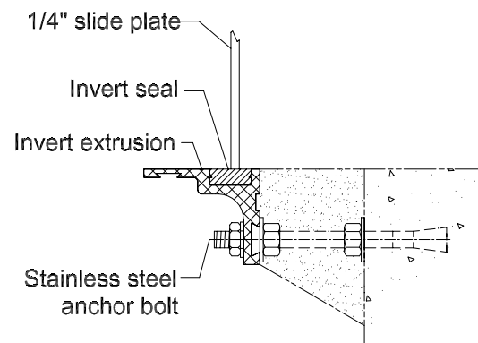
FLUSH BOTTOM INVERT * Detail-C
