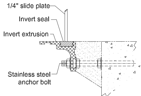
FLUSH BOTTOM INVERT Detail-B
