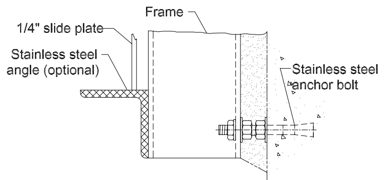
GATE STOP ANGLE (optional) * Detail-C
