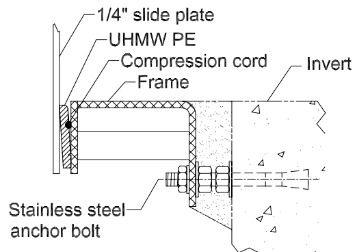
INVERT SEAL * Detail-B
