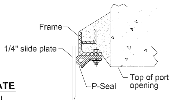
UPPER SEAL Detail-B
