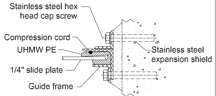
GUIDE FRAME Detail-A
