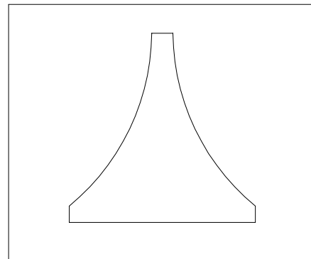
PROPORTIONAL WEIR PLATE
