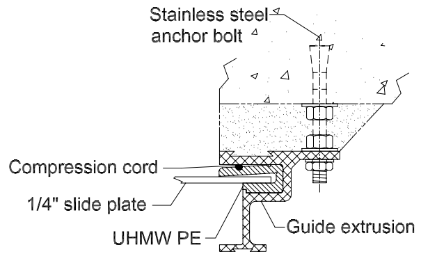
GUIDE FRAME * Detail-A
