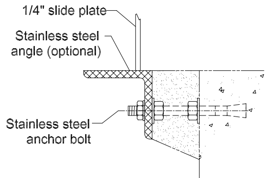
GATE STOP ANGLE (optional) Detail-C
