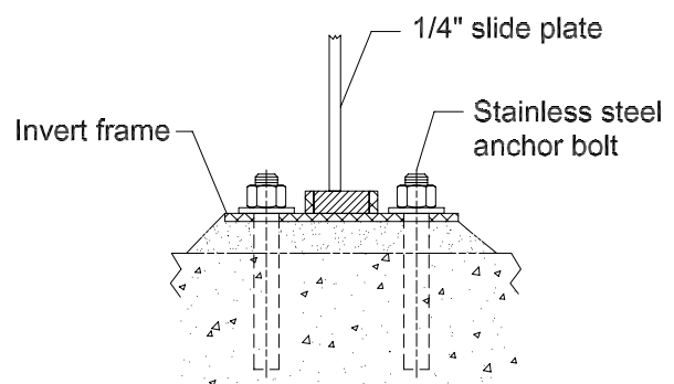
INVERT (OPTION 2) Detail-B
