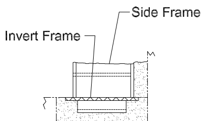
FLUSH BOTTOM INVERT Detail-C
