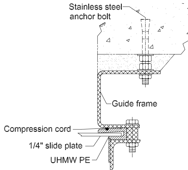
GUIDE FRAME * Detail-A
