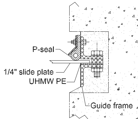
GUIDE FRAME Detail-A
