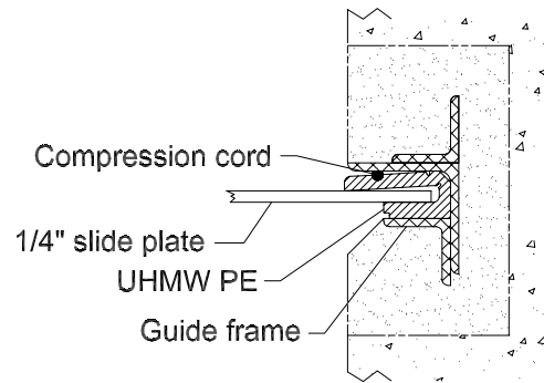
GUIDE FRAME Detail-A
