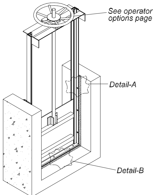
SELF-CONTAINED GATE WITH BENCH (YOKE)
