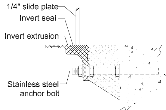
FLUSH BOTTOM INVERT Detail-C
