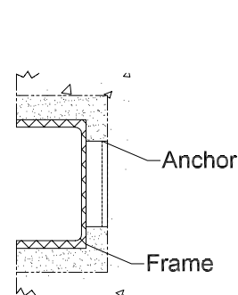
EMBEDDED Detail-A
