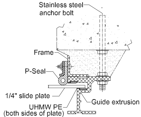
GUIDE FRAME Detail-A
