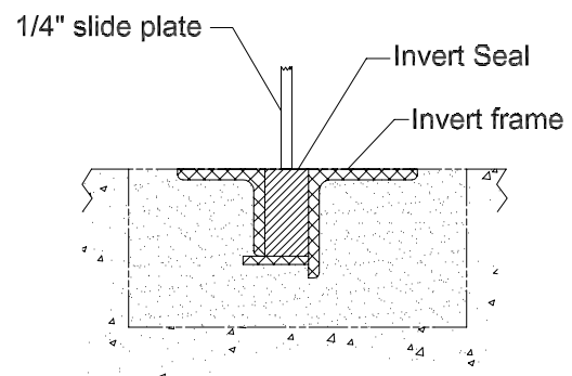
FLUSH BOTTOM INVERT Detail-B
