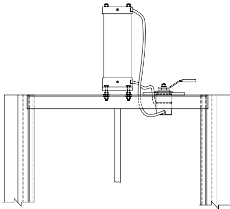
HYDRAULIC/PNEUMATIC ACTUATOR (Bench Mount)
