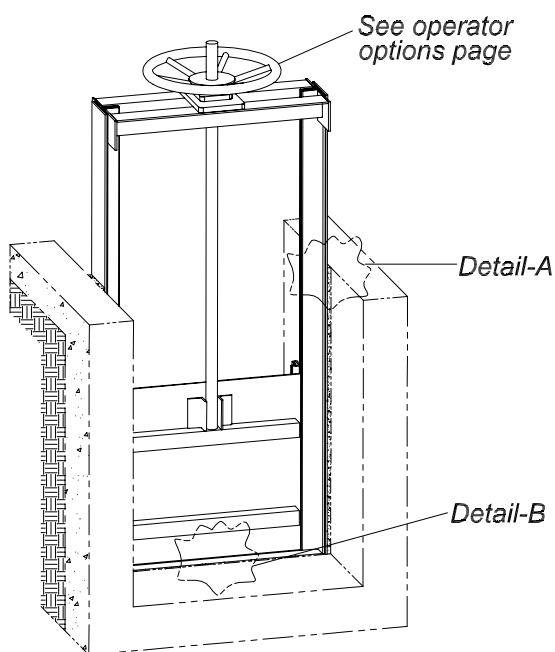
SELF-CONTAINED GATE WITH BENCH (YOKE)
