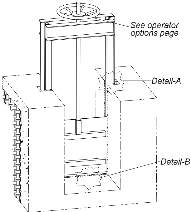
SELF-CONTAINED GATE WITH BENCH (YOKE)
