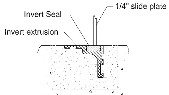
FLUSH BOTTOM INVERT Detail-B
