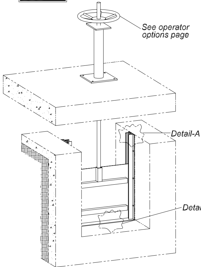
NON-SELF-CONTAINED GATE WITH FABRICATED PEDESTAL
