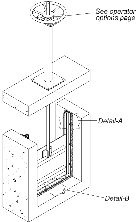
NON-SELF-CONTAINED GATE WITH FABRICATED PEDESTAL
