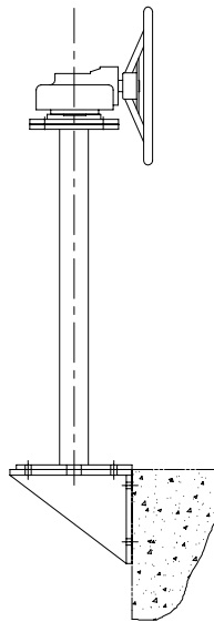
Wall Bracket (with pipe pedestal and BS2000 handwheel)
