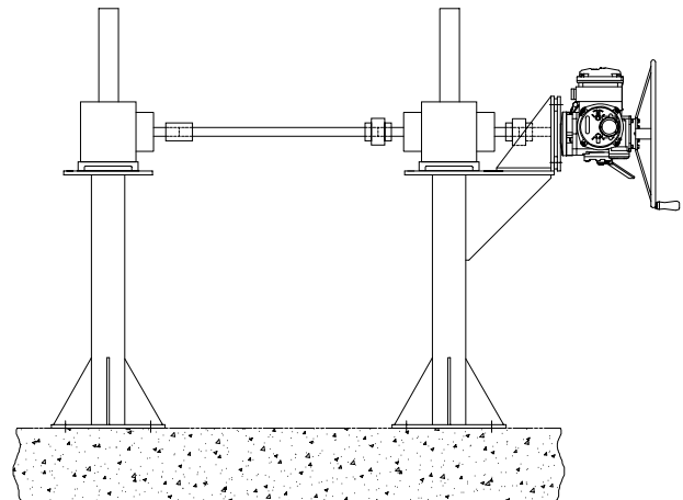
DUAL STEM PEDESTAL (with Electric Actuator)
