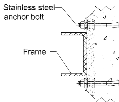
CHANNEL SURFACE * Detail-A
