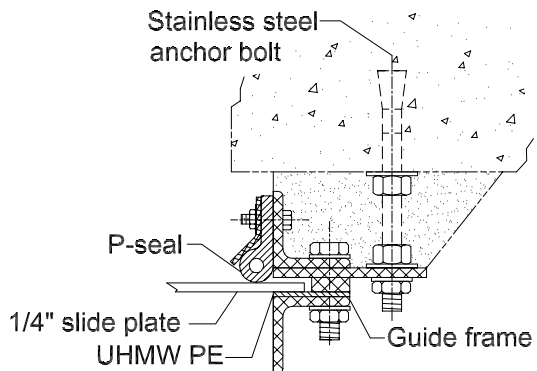
GUIDE FRAME Detail-A
