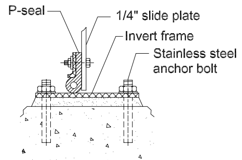
INVERT (OPTION 1) Detail-B
