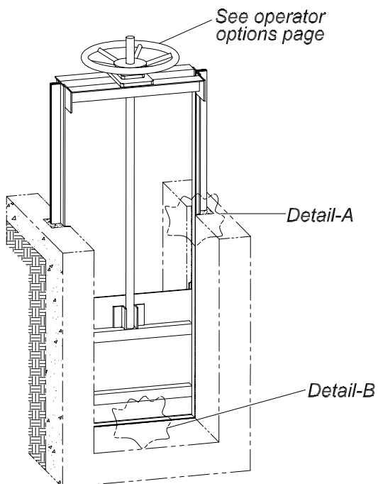
SELF-CONTAINED GATE WITH BENCH (YOKE)
