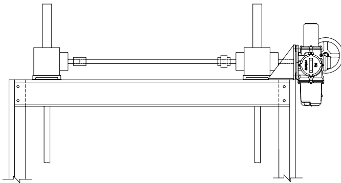
DUAL STEM OPERATOR (with Electric Actuator)
