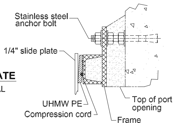
UPPER SEAL * Detail-B
