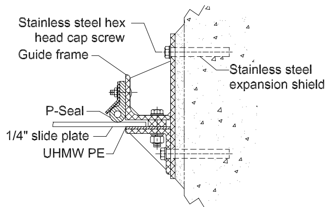
GUIDE FRAME Detail-A
