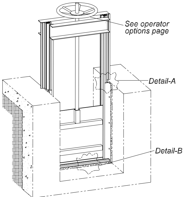
SELF-CONTAINED GATE WITH BENCH (YOKE)
