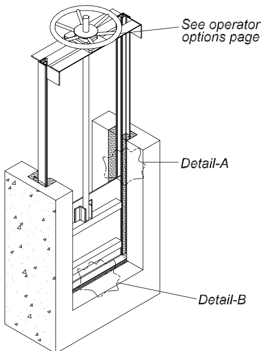
SELF-CONTAINED GATE WITH BENCH (YOKE)
