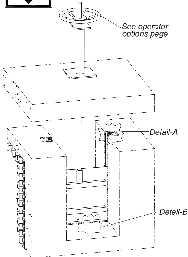
NON-SELF-CONTAINED GATE WITH FABRICATED PEDESTAL
