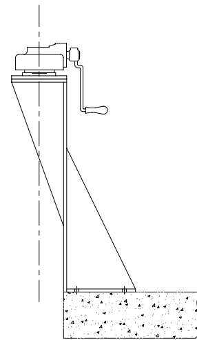
Offset Pedestal (with BS2000 handcrank)
