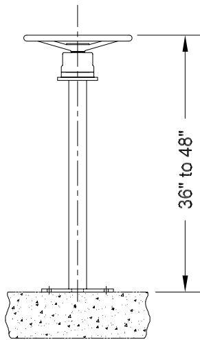
Standard Pipe Pedestal (with BS1015)
