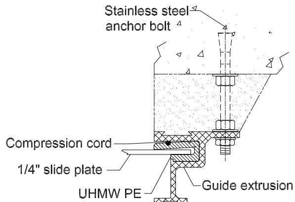
GUIDE FRAME * Detail-A
