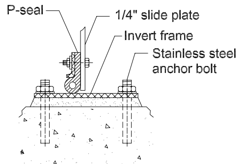
INVERT (OPTION 2) Detail-B
