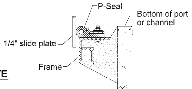
INVERT SEAL Detail-B
