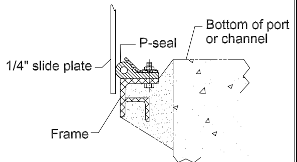
INVERT SEAL Detail-B
