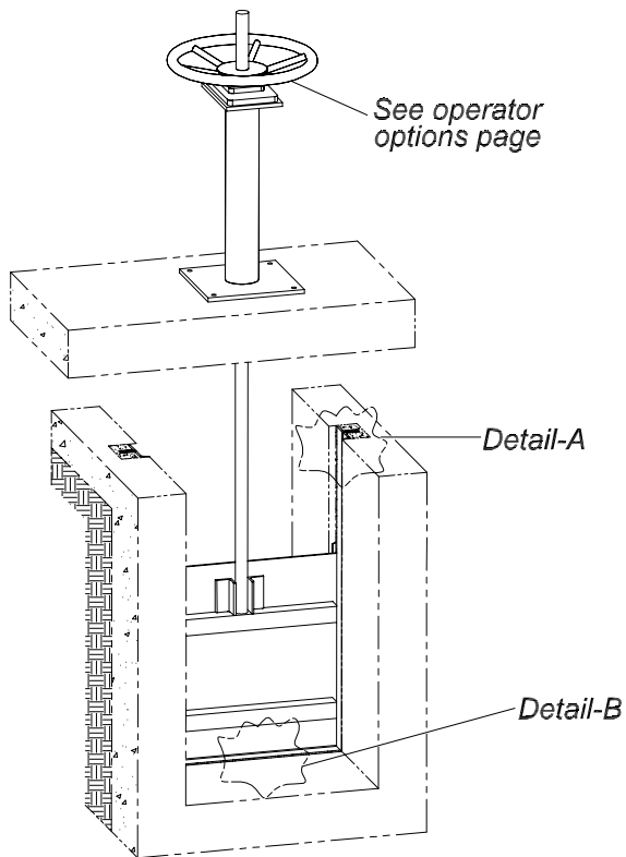
NON-SELF-CONTAINED GATE WITH FABRICATED PEDESTAL
