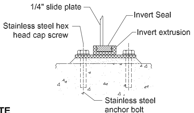
INVERT (OPTION 2) Detail-B
