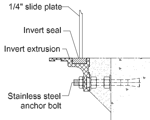
FLUSH BOTTOM INVERT * Detail-B
