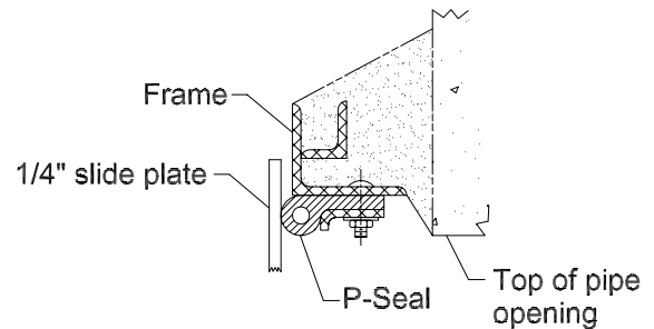
UPPER SEAL Detail-B
