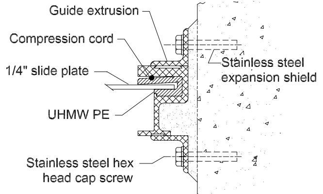
GUIDE FRAME Detail-A
