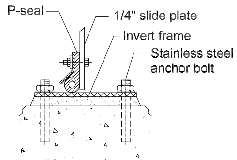
INVERT (OPTION 1) Detail-B
